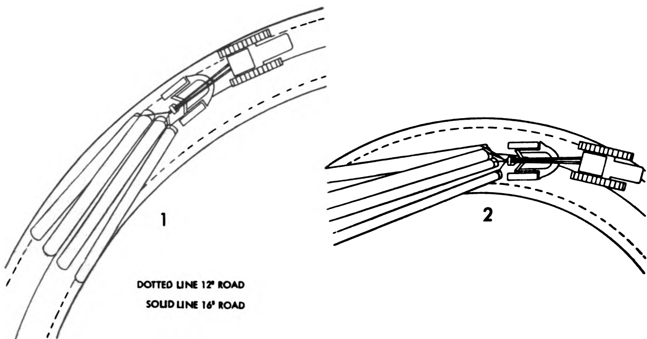
Figure 4-1. Lengthening a curve for tractor-arch logging.
